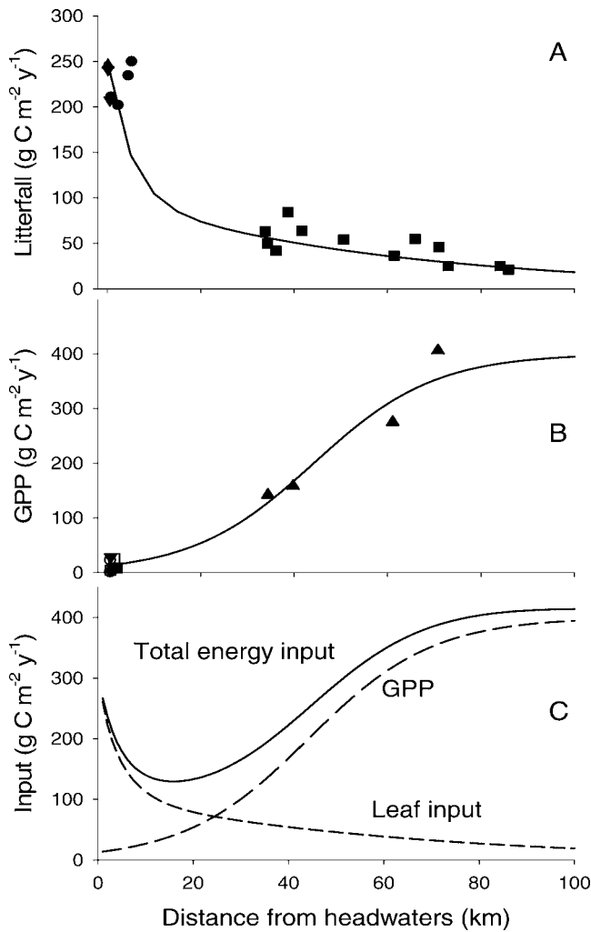
FIG. 3. Litterfall input (A), gross primary production (GPP) (B), and total energy inputs (U-shaped curve) (C) in the Little Tennessee River. Lines in (A) and (B) are regression lines (litterfall: negative exponential, r^2 = 0.94 ; GPP: sigmoid function, r^2 = 0.97 ). All litterfall data are annual estimates as reported by the authors. All GPP values are 1-time measurements except for the annual values reported by McTammany et al. (2003). Leaf input in (C) includes lateral input from Webster and Waide (1982), Webster et al. (1990), and Wallace et al. (1997). Regression line for GPP (sigmoid function, r^2 = 0.97 ) is fit to data of Hains 1981 (circles); Mulholland et al. 1997 (triangle down); McTammany et al. 2003 (triangles up); Webster et al. 2003 (square); H. M. Valett, Virginia Polytechnic Institute and State University, S. A. Thomas, University of Nebraska, and JRW, unpublished data (open circles); JRW, H. M. Valett, and B. R. Niederlehner, Virginia Polytechnic Institute and State University, unpublished data (open squares).
