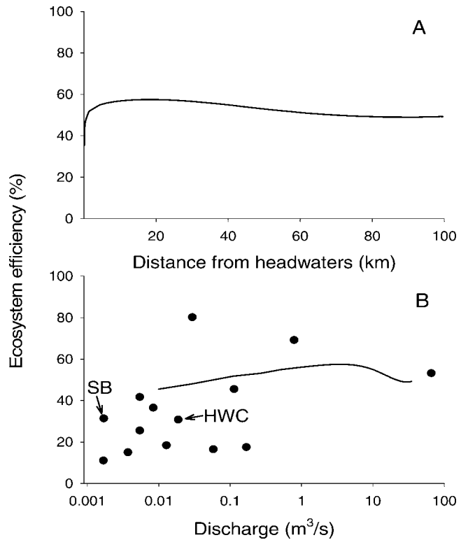
FIG. 11. A.—Ecosystem efficiency along the Little Tennessee River. B.—Comparison of model-estimated ecosystem efficiency (solid line) and stream efficiencies estimated by Webster and Meyer (1997; watershed budgets only, outliers identified by Webster and Meyer 1997 are not included). Satellite Branch (SB) and Hugh White Creek (HWC) are streams at Coweeta.
