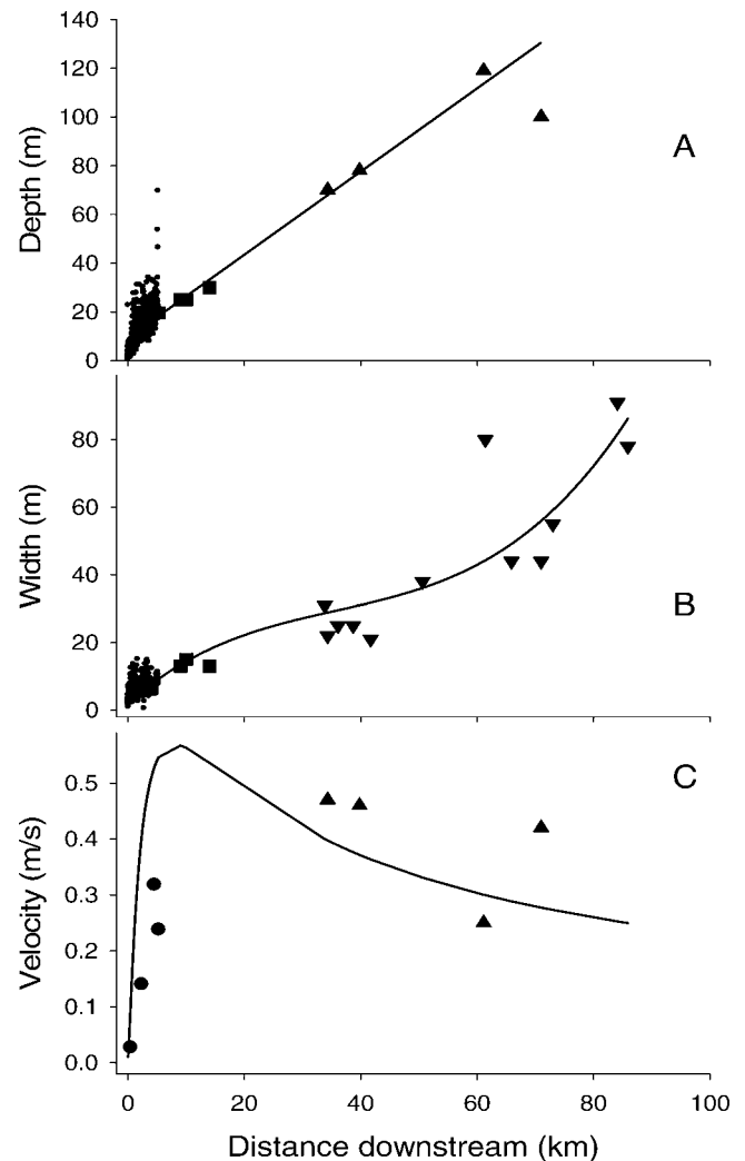
FIG. 2. Depth (A), width (B), and average velocity (C) in the Little Tennessee River. Velocity (line) was calculated from discharge (Fig. 1B), depth, and width. Lines in (A) and (B) are regression lines (depth: linear, r^2 = 0.80 ; width: 3 rd -order polynomial, r^2 = 0.73 ). Depth and width data are from JRW, J. B. Wallace, University of Georgia, J. L. Meyer, University of Georgia, E. F. Benfield, University of Georgia, and G. D. Grossman, University of Georgia, unpublished data (circles); Grubaugh et al. 1997 (squares); Neatrour et al. 2004 (triangles down); and McTammany et al. 2003 (triangles up). Data points in (C) are measurements of D'Angelo et al. 1993 (circles) and McTammany et al. 2003 (triangles).
