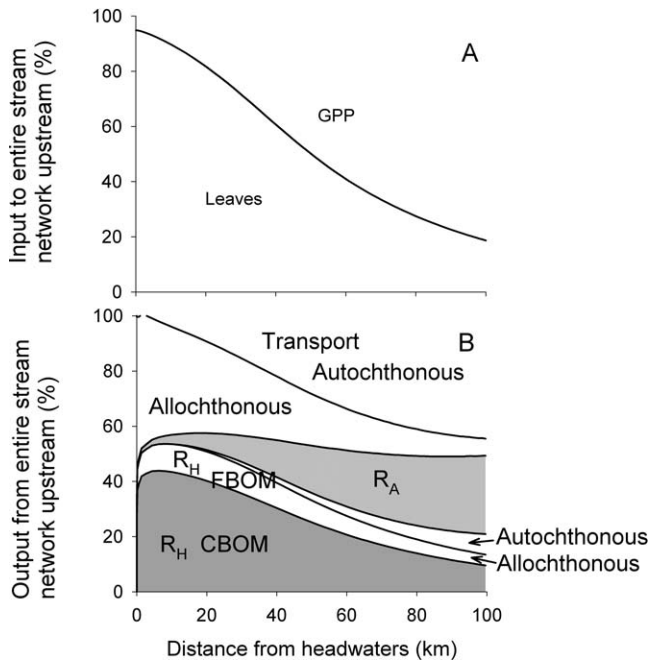
FIG. 10. Changes in the particulate organic matter budget along the Little Tennessee River. At each point along the length of the stream, the estimates of input (A) and output (B) are for the stream network upstream of that point. Respiration is divided into 3 components: autotrophic respiration ( R_A ), heterotrophic respiration ( R_H ) of coarse benthic organic matter (CBOM), and R_H of fine benthic organic matter (FBOM). Transport and R_H of FBOM are also separated based on the allochthonous or autochthonous source of the material. GPP = gross primary production.
