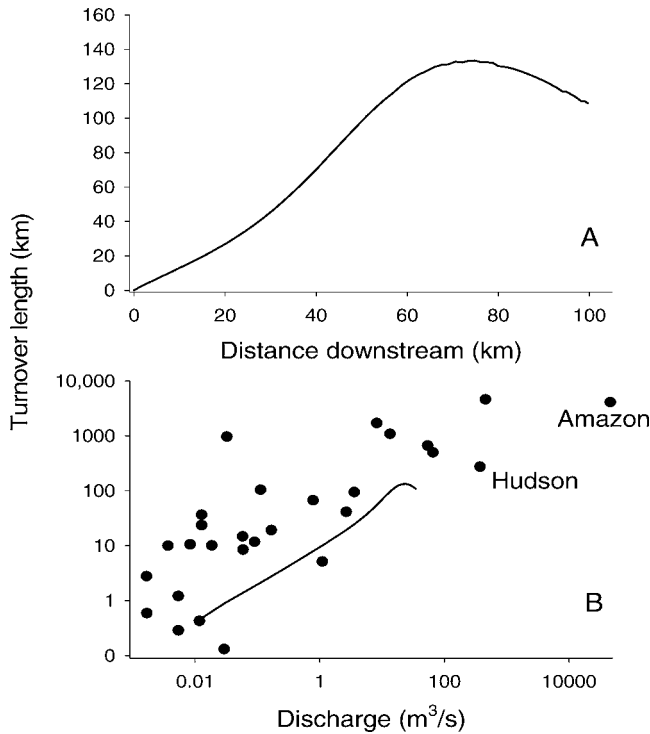
FIG. 12. A.—Turnover length along the Little Tennessee River. B.—Comparison of model-estimated turnover length (solid line) and turnover lengths estimated by Webster and Meyer (1997), Richey et al. (1990; Amazon River), and Howarth et al. (1996; Hudson River).
