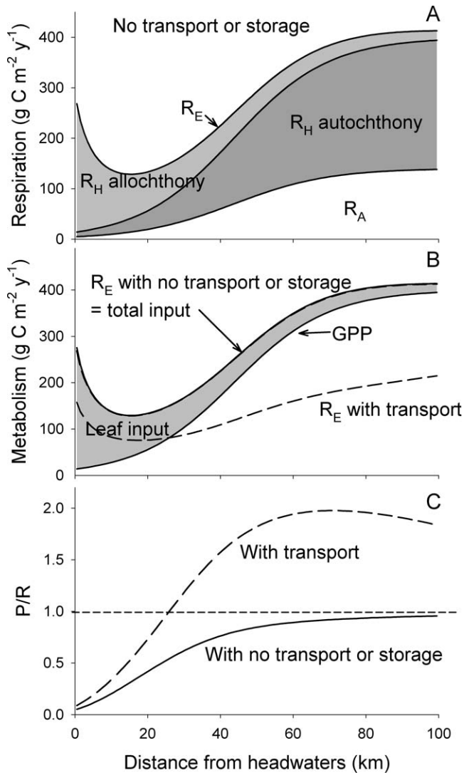
FIG. 13. A.—Simulated respiration in the Little Tennessee River (LTR) with no transport and no storage. Components of respiration are autotrophic respiration ( R_A ), ecosystem respiration ( R_E , upper line), and heterotrophic respiration ( R_H , shaded area). R_H is divided into respiration of allochthonous material and autochthonous material. B.—Simulated metabolism in the LTR. The top solid line is total input, which is equal to R_E in this simulation, and the lower solid line is gross primary production (GPP). The shaded area between the solid lines is leaf input. For comparison, the dashed line is ecosystem respiration ( R_E ) in the normal simulation with transport. C.—Comparison of production (P)/respiration (R) ratios with and without transport.
