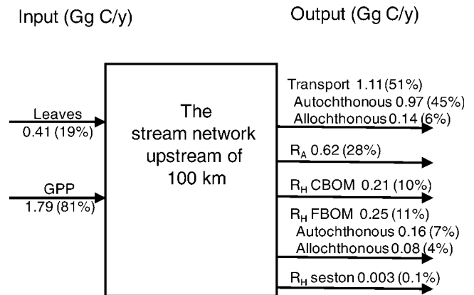
FIG. 9. Particulate organic matter budget for the Little Tennessee River network upstream of 100 km. Transport and heterotrophic respiration ( R_H ) of fine benthic organic matter (FBOM) are separated based on the allochthonous or autochthonous source of the material. Percentages shown in parentheses are based on % of total inputs or outputs. Gg = 10^9 g, CBOM = coarse benthic organic matter, R_A = autotrophic respiration.
