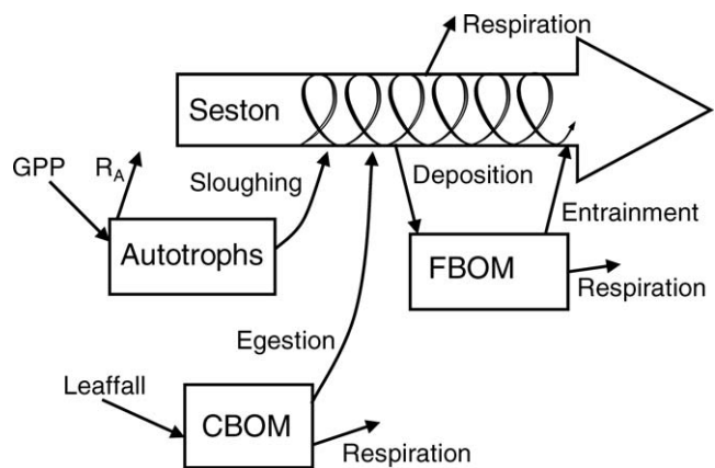
FIG. 4. Compartment model of particulate organic matter dynamics in the Little Tennessee River. GPP = gross primary production, R_A = autotrophic respiration, CBOM = coarse benthic organic matter, FBOM = fine benthic organic matter.
