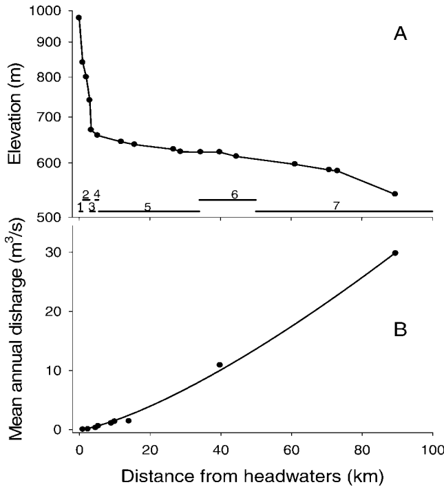
FIG. 1. A.—Gradient of the Little Tennessee River (LTR) based on elevations read from 1:24,000-scale US Geological Survey (USGS) maps. Bars at the bottom of the figure indicate stream order (see text). B.—Average annual discharge in the LTR (data are from US Forest Service, Coweeta Hydrologic Laboratory, Otto, North Carolina, and USGS, http://waterdata.usgs.gov/nc/nwis ). Regression line in (B) is a power function ( r^2 = 0.997 ).
