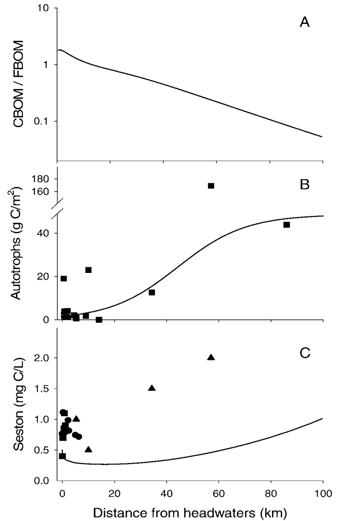
FIG. 6. Coarse benthic organic matter (CBOM)/fine benthic organic matter (FBOM) ratio (A) and autotroph (B) and seston (C) standing crops in the Little Tennessee River. Lines are results of model simulations. Data from Grubaugh et al. 1997 (squares) and JRW, E. F. Benfield, Virginia Polytechnic Institute and State University, and J. L. Tank, University of Notre Dame, unpublished (circles) are annual averages calculated from seasonal samples. The data from JRW, H. M. Valett, Virginia Polytechnic Institute and State University, and B. R. Niederlehner, Virginia Polytechnic Institute and State University, unpublished (open squares) are single measurements. Data from Grubaugh et al. (1997) are weighted averages from the various sampled habitats. All seston data are annual averages as reported by the authors. Seston data are from Wallace et al. 1982b (circles); Webster and Golladay 1984 (squares); and Rosi-Marshall and Meyer 2004 (triangles).
