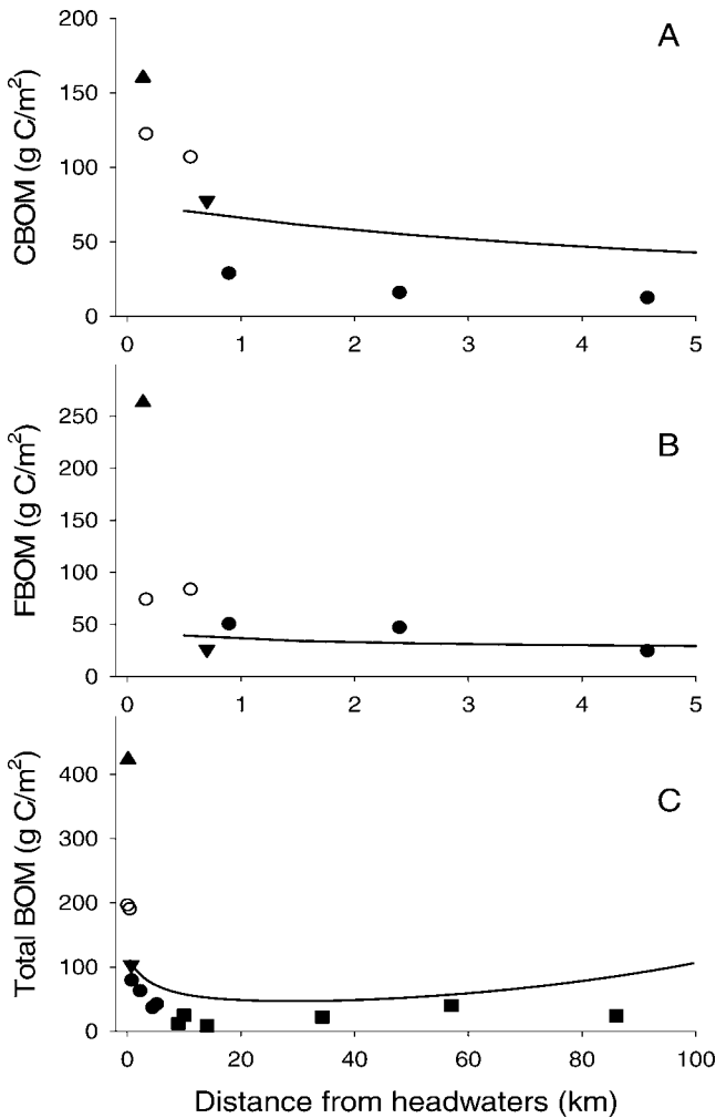
FIG. 5. Coarse benthic organic matter (CBOM) (A), fine benthic organic matter (FBOM) (B), and total benthic organic matter (BOM) (C) standing crops in the Little Tennessee River. CBOM and FBOM are shown only for the first 5 km to illustrate the major changes occurring in the upper reaches of the river. Lines are results of model simulations. All data are annual averages as calculated by the authors. Data from Grubaugh et al. (1997) are based on BOM in depositional areas and % depositional area of the river. Data points are from Grubaugh et al. 1997 (squares), Huryn and Wallace 1987 (triangles down), Golladay et al. 1989 (open circles), Wallace et al. 1997 (triangles up), and Benfield et al. 2000 (solid circles).
