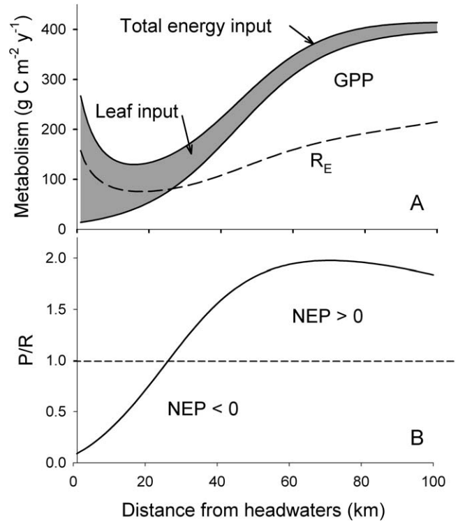
FIG. 8. A.—Simulated metabolism in the Little Tennessee River. The top solid line is total input and the lower solid line is gross primary production (GPP). The shaded area between the solid lines is leaf input. The dashed line is ecosystem respiration ( R_E ). B.—Production (P)/respiration (R) ratio corresponding to the simulated metabolism results. Dashed line shows P/R = 1 for reference. Where GPP > R_E , net ecosystem production (NEP) > 0 and where GPP < R_E , NEP < 0 .
