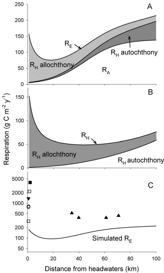
FIG. 7. A.—Simulated components of respiration in the Little Tennessee River are autotrophic respiration ( R_A ), ecosystem respiration ( R_E , upper line), and heterotrophic respiration ( R_H , shaded area). R_H is divided into respiration of allochthonous material and autochthonous material. B.—The U-shaped curve of R_H . C.—Simulated and measured values of R_E . All values are one-time measurements except for the annual values reported by McTammany et al. (2003). Measurements of ecosystem respiration are from Mulholland et al. (1997, triangle down); McTammany et al. (2003, triangles up); Webster et al. (2003, solid square); H. M. Valett, Virginia Polytechnic Institute and State University, S. A. Thomas, University of Nebraska, and JRW, unpublished data (open circle); and JRW, H. M. Valett, and B. R. Niederlehner, Virginia Polytechnic Institute and State University, unpublished data (open square).
