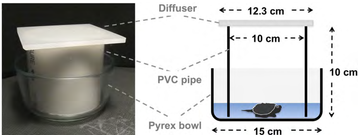
Fig 2. The experimental chamber. Turtles were tested in a Pyrex bowl with water that was \sim 1 cm deep so the turtle's shell was not completely submerged. The Pyrex bowl, PVC surround, and overhead diffuser provided uniform visual surroundings.
